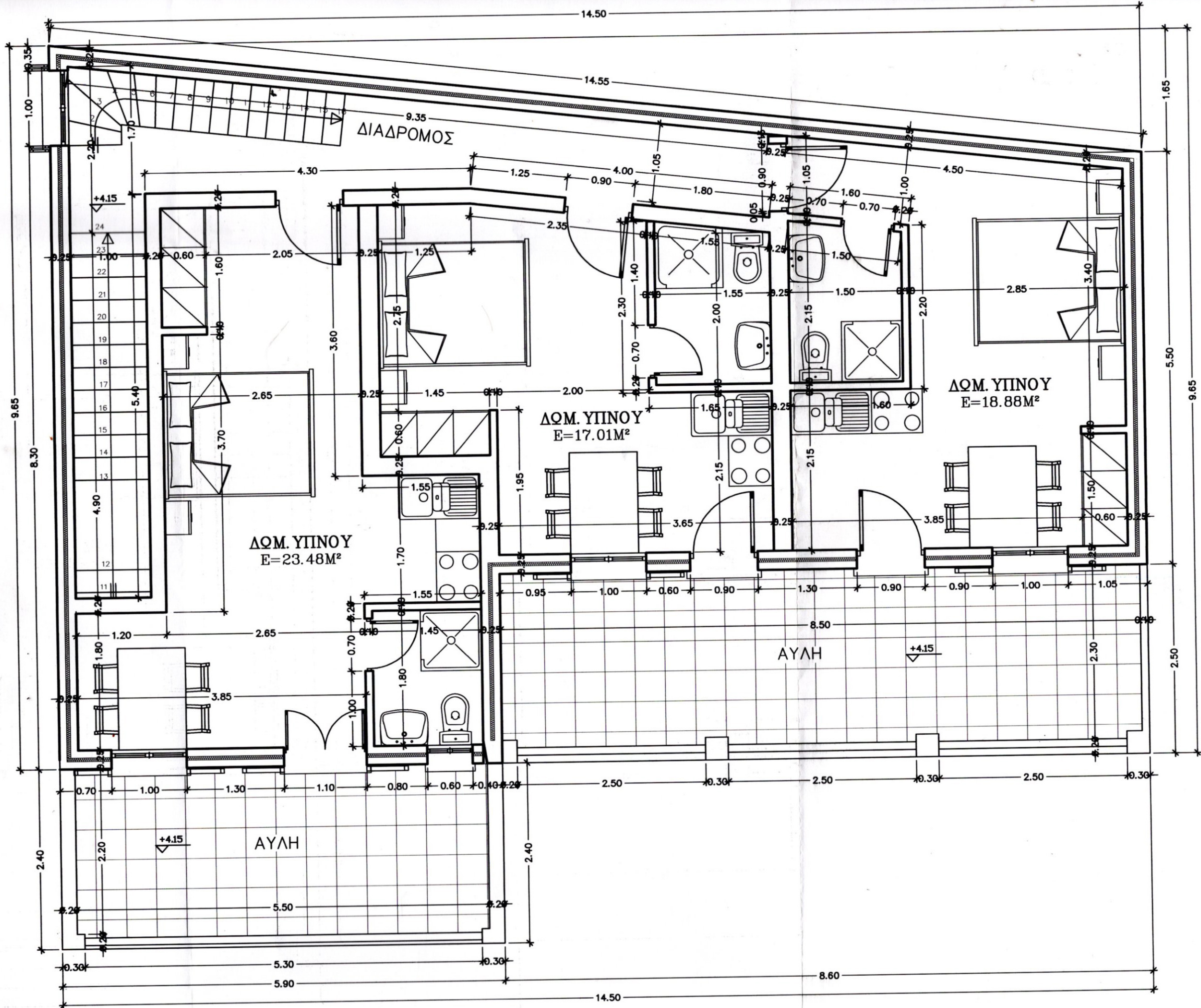
ΟΡΟΦΟΣ/FIRST FLOOR
